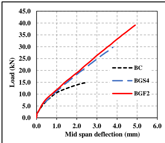
Fig. 6. Load versus Mid span deflection.
