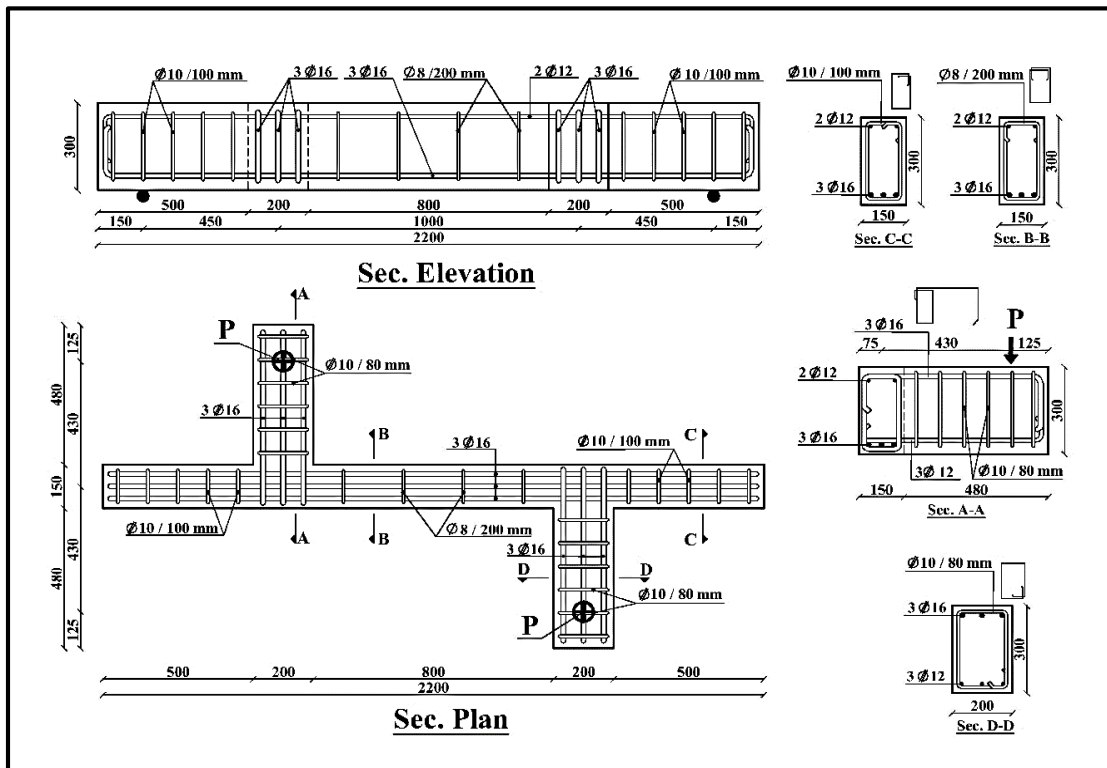
Fig. 1. Dimensions and reinforcement details of test beam.
