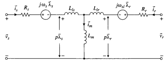
Fig. 3 DFIG equivalent circuit in the synchronous frame
